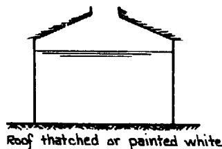
Fig. 11 - ROOFS FOR TANKS LESS THAN 5 M. DIA.
