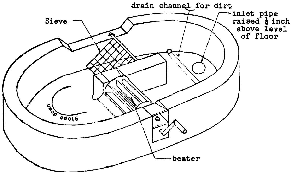
Slurry-mixing machine
