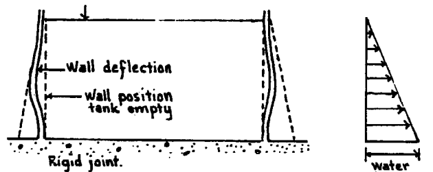
Fig. 8 WALLS JOINED WITH FLOOR
